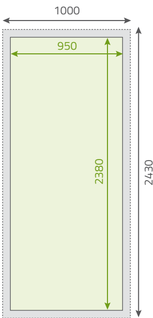
① Standardwand
